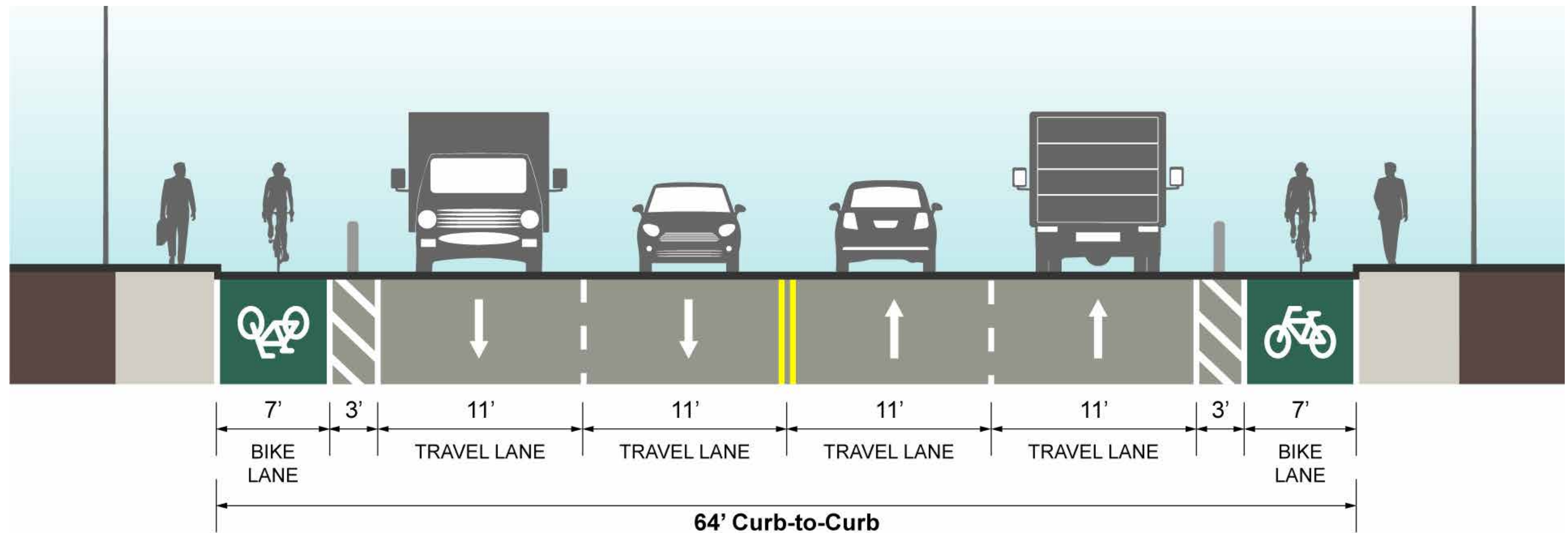
Figure 31: Concept D: Four Travel Lanes, No Parking
