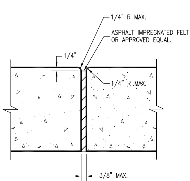
EXPANSION JOINT
