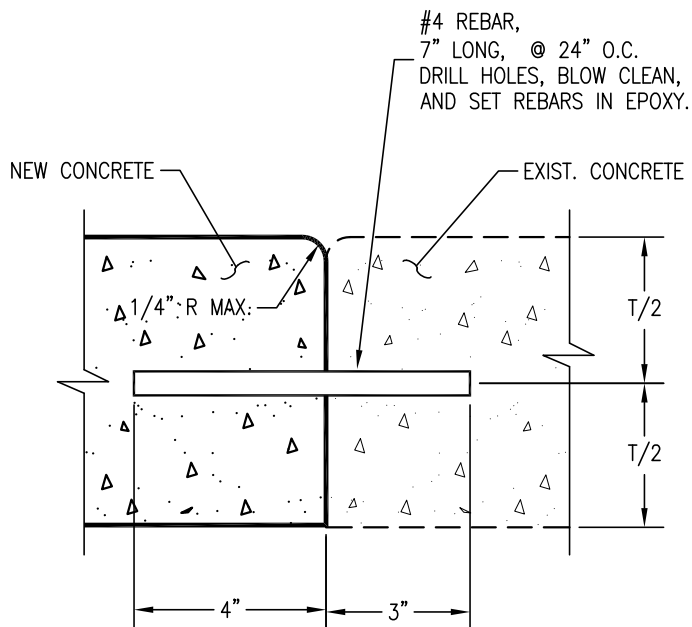
SIDEWALK CONTACT JOINT "COLD JOINT"
