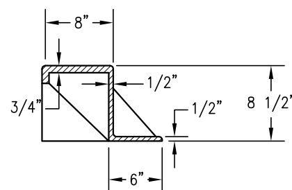
SECTION A-A NO SCALE
