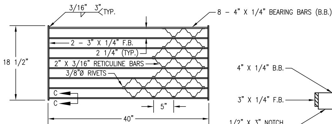
GRATE — PLAN VIEW NO SCALE
