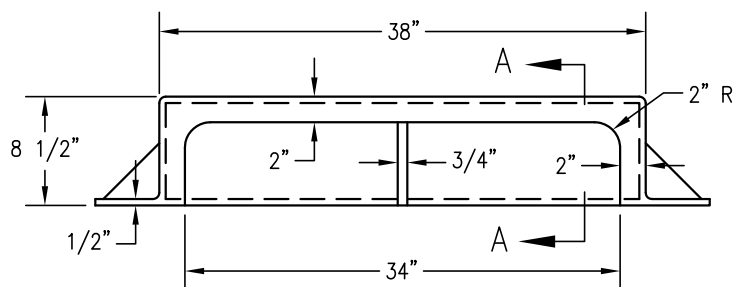
HOOD — FRONT VIEW NO SCALE
