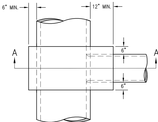
PERPENDICULAR CONNECTION PLAN VIEW NO SCALE
