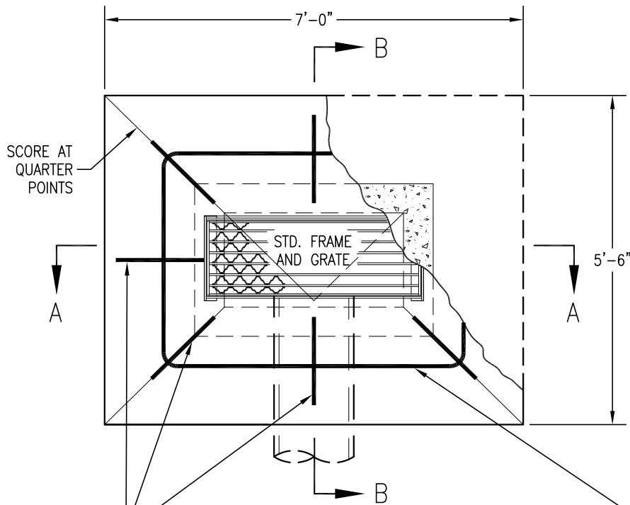
PLAN VIEW NO SCALE
