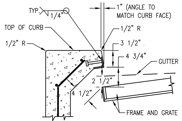
FACE ANGLE ANCHOR DETAIL NO SCALE
