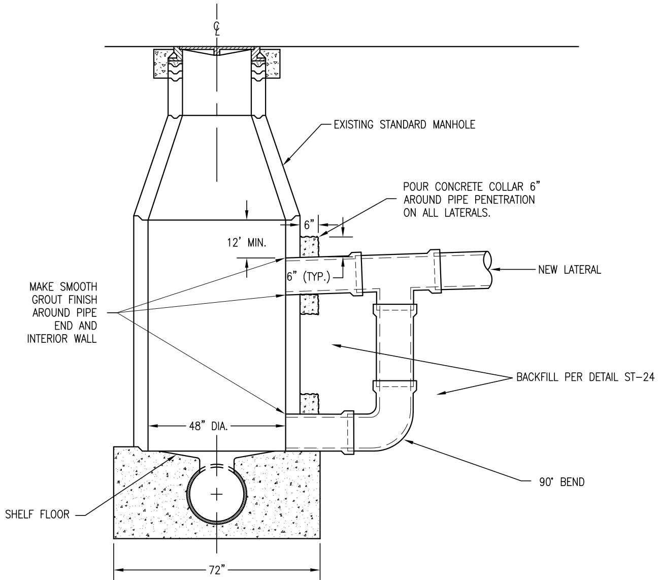
ELEVATION VIEW NO SCALE
