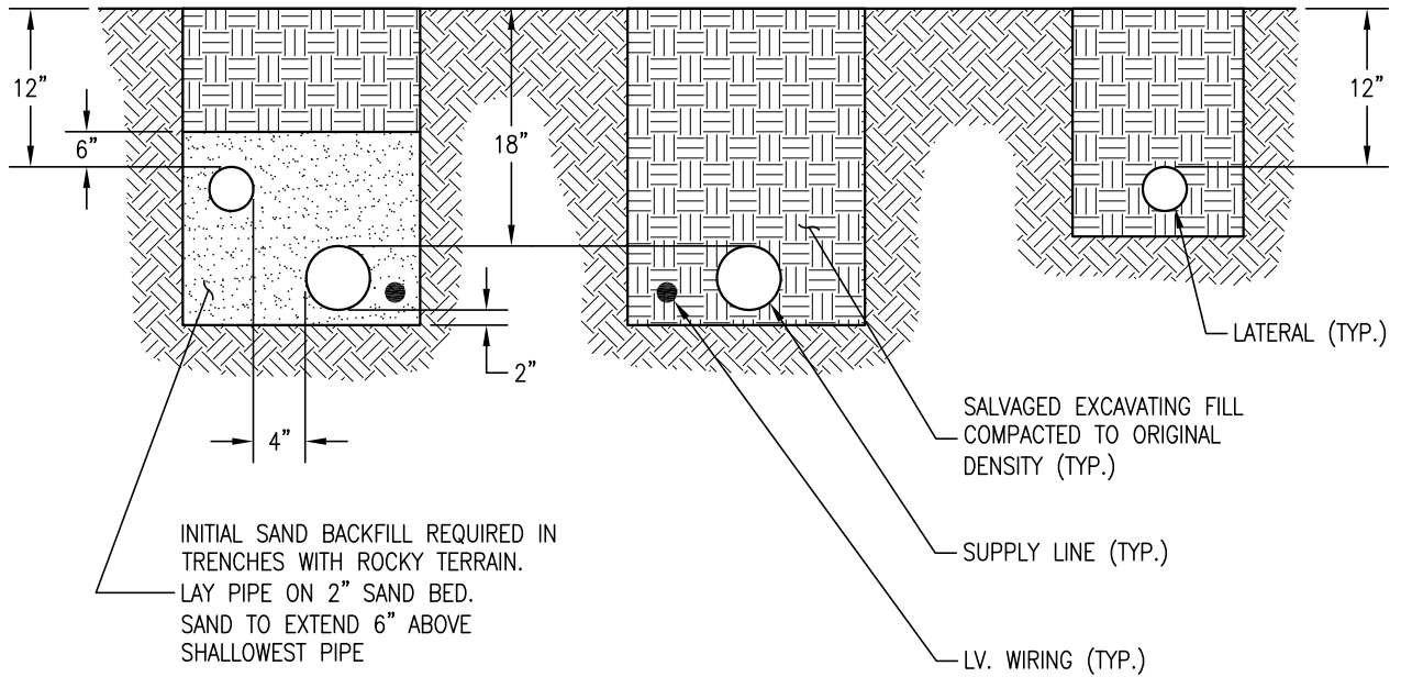
TRENCHES IN PLANTING AREA ELEVATION VIEW NO SCALE
